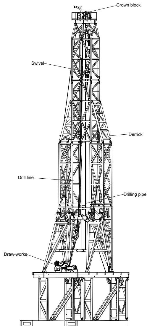
Figure 1: Drilling Rig scheme
